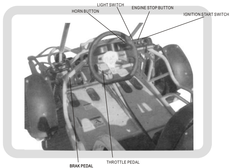
Figure 1 front panel
