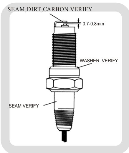
Figure 6 Spark plug
