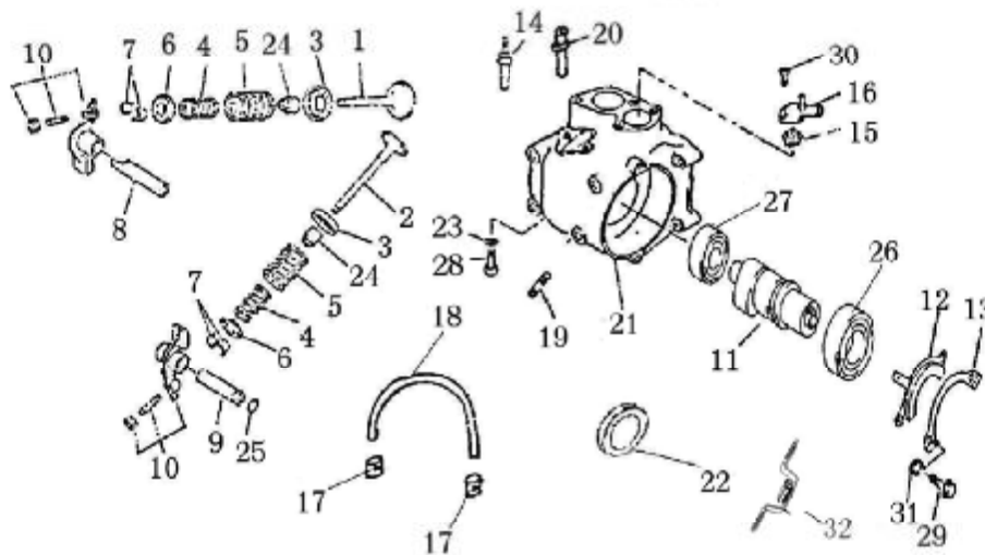
FIG. 4 CYLINDER HEAD COMP.
