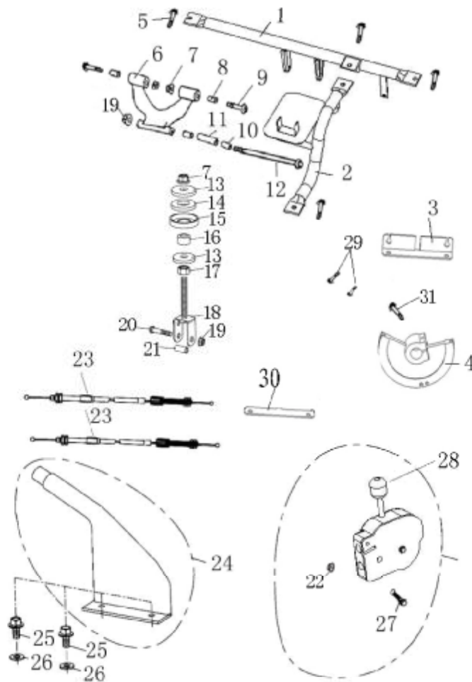
FIG. 16 FULL SHIFTING ASSY.
