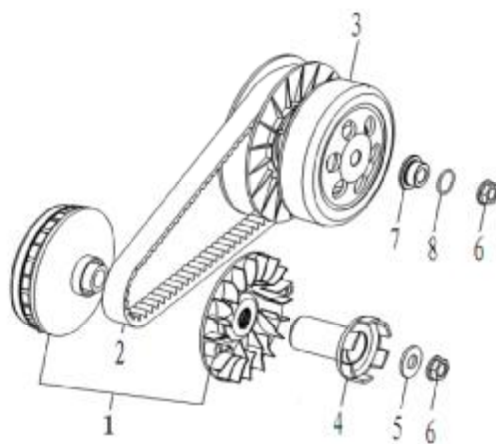
FIG. 7 V-BELT DRIVING
