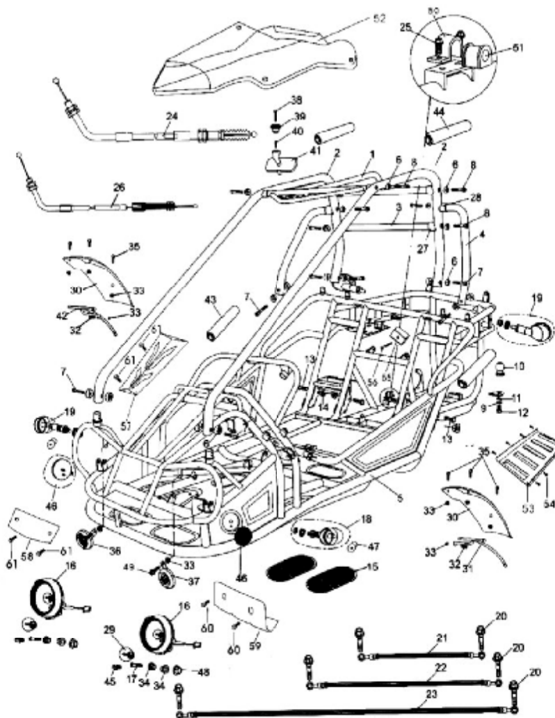
FIG. 13 FRAME GROUP
