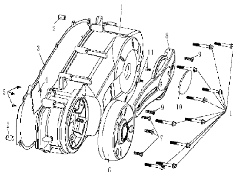
FIG. 9 JINGLANG TYPE-RUYI LEFT COVER COMP. (169.03.400B)
