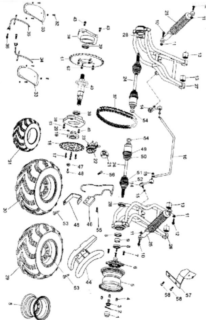
FIG. 19 REAR SUSPENSION ASSY.
