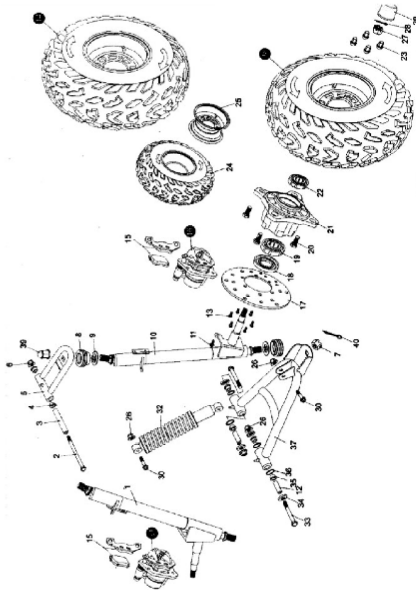
FIG. 15 FRONT SUSPENSION ASSY.
