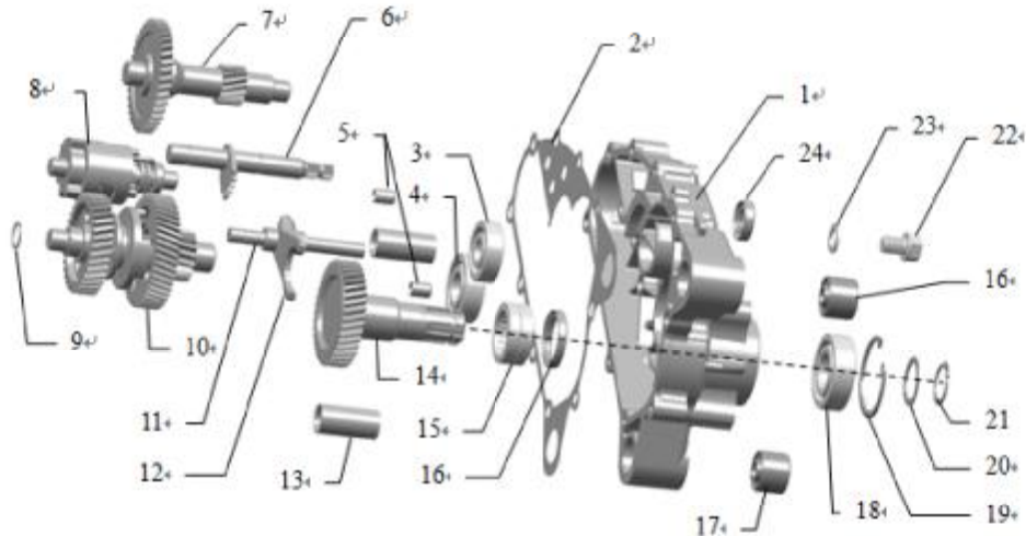
FIG. 8 GEARBOX DRIVING
