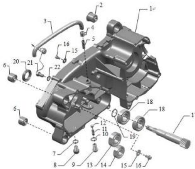
FIG. 1 LEFT CRANKCASE COMP.
