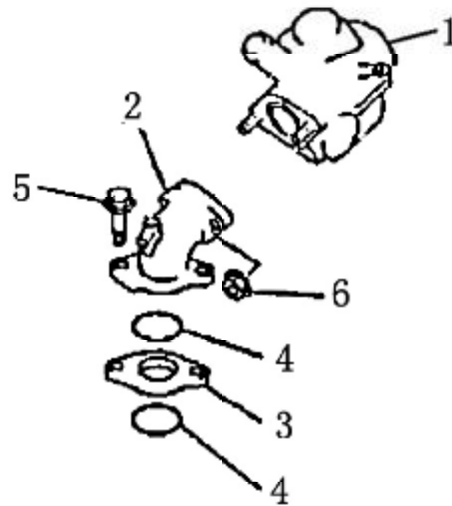
FIG. 10 INTAKE PIPE, CARBURETOR
